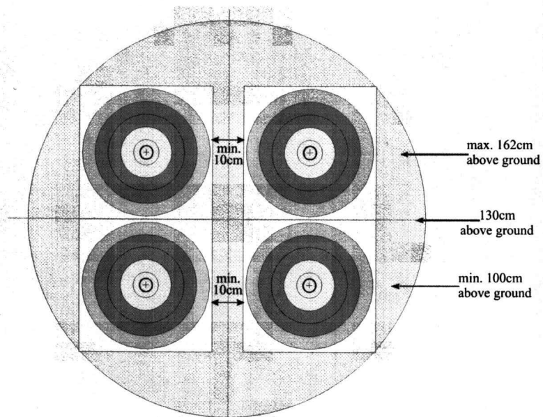
80cm-center four-center set-up
